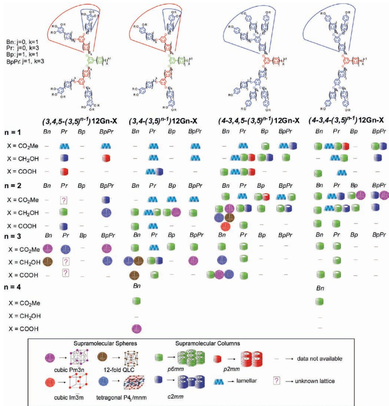
Figure 14. Primary structure vs 3D supramolecular structure for all 3,5-disubstituted libraries of AB 2 supramolecular dendrimers. Bn = benzyl ether, Pr = phenylpropyl ether, Bp = biphenyl-4-methyl ether, BpPr = biphenylpropyl ether.
