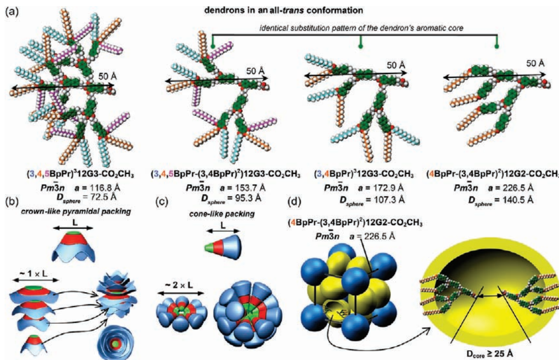
Figure 7. Molecular models of the four chosen dendrons in the all-trans conformation (a), crown-like pyramidal packing proposed for (3,4,5\text{BpPr})^3 12\text{G3-CO}_2\text{CH}_3 (b), cone-like packing proposed for (3,4,5\text{BpPr-(3,4BpPr)}_2) 12\text{G3-CO}_2\text{CH}_3 and (3,4\text{BpPr})^3 12\text{G3-CO}_2\text{CH}_3 (c). Unit cell and to-scale molecular model of (4\text{BpPr-(3,4BpPr)}_2) 12\text{G2-CO}_2\text{CH}_3 depicting the lower bound of the empty core diameter D_{\text{core}} (d).
