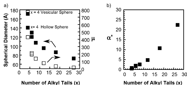
Figure 8. Effect the number of alkyl tails ( x ) on the spherical diameter and on the number of dendrons per supramolecular dendritic sphere ( \mu ) generated from third generation dendrons or dendrons of comparable molecular dimensions (a). Dependence of the calculated projection of the solid angle ( \alpha' ) of the dendrons in the supramolecular sphere on the number of alkyl tails ( x ) (b).
