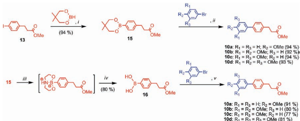
Scheme 3. Expedient Four and Five Step Synthesis of BpPr Building Blocks Utilizing One Boronic Acid a
