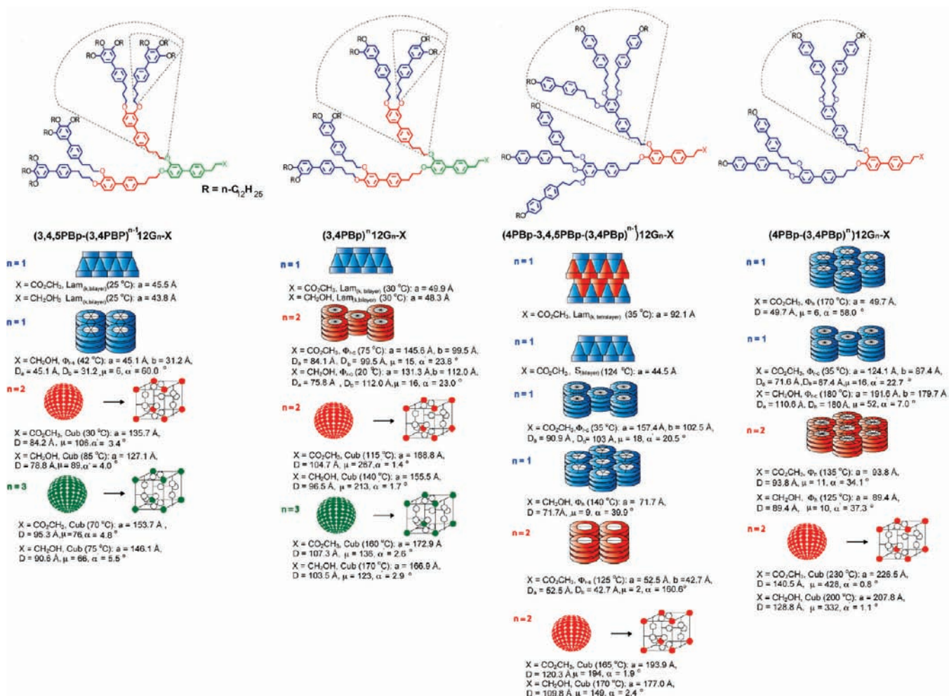
Figure 3. Structural and retrostructural analysis of supramolecular dendrimers self-assembled from AB 2 3,4-disubstituted dendrons.
