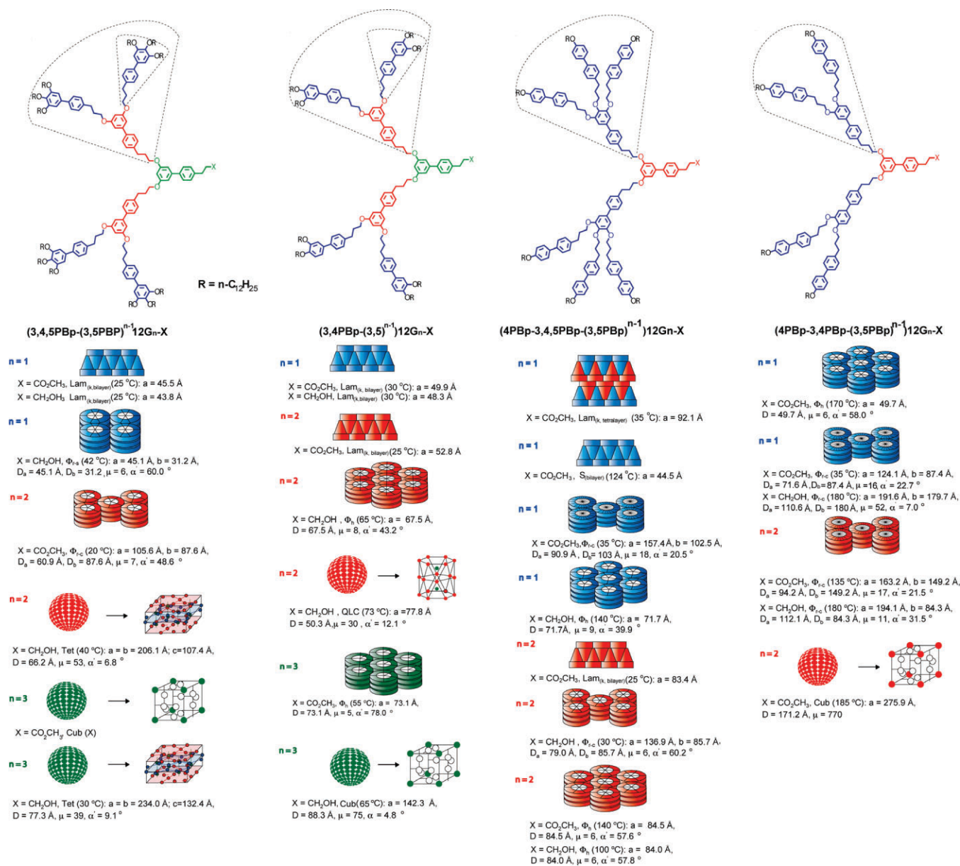
Figure 4. Structural and retrostructural analysis of supramolecular dendrimers self-assembled from AB 2 3,5-disubstituted dendrons.
