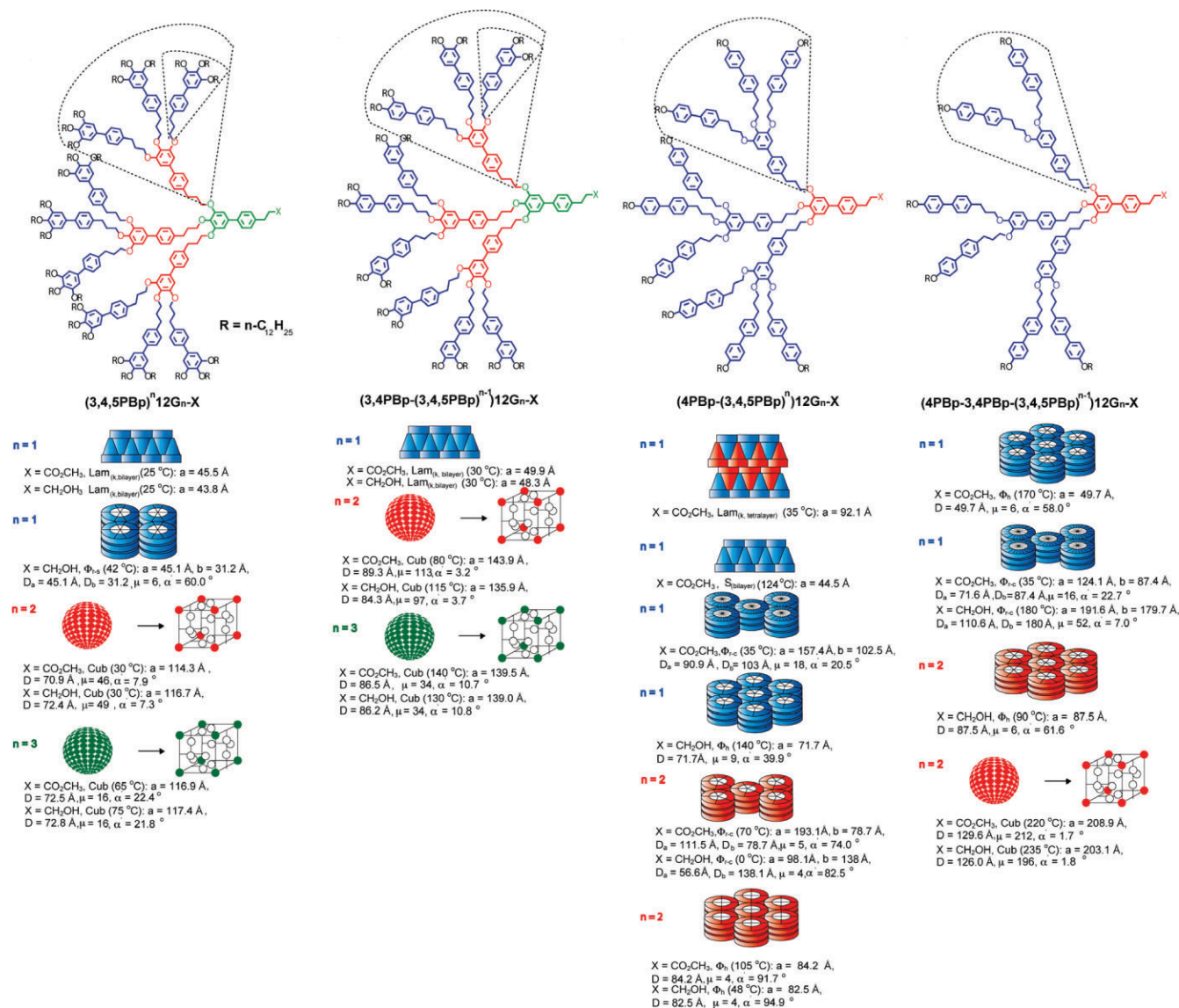
Figure 2. Structural and retrostructural analysis of supramolecular dendrimers self-assembled from AB 3 3,4,5-trisubstituted dendrons.
