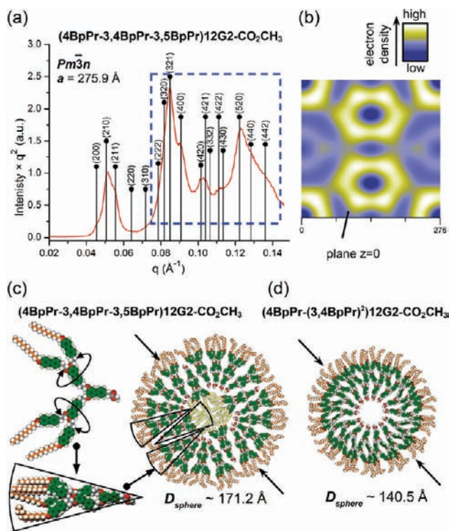
Figure 9. Vesicular cubic phase: (4BpPr-3,4BpPr-3,5BpPr)12G2-CO 2 CH 3 XRD powder plot with the increased relative intensities of the high order peaks marked by the dotted rectangle (a), corresponding relative electron density map (b), corresponding model of the self-assembled vesicular sphere (c), and comparison with the model of the hollow cubic spheres self-assembled from (4BPb-(3,4BPb) 2 )12G2-CO 2 CH 3 (d).
