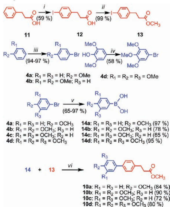
Scheme 2. Improved Four Step Synthesis of BpPr Dendritic Building Blocks a
