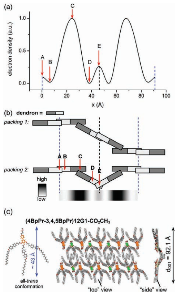
Figure 5. Lamellar crystalline structure with four layer repeat observed for (4BpPr-3,4,5BpPr)12G1-CO 2 CH 3 . (a) Electron density map indicating decreased electron density in every other layer. (b) Proposed packing models together with the electron density map. (c) Molecular model of (4BpPr-3,4,5BpPr)12G1-CO 2 CH 3 and the top and side view of the puckered tetralayer model.
