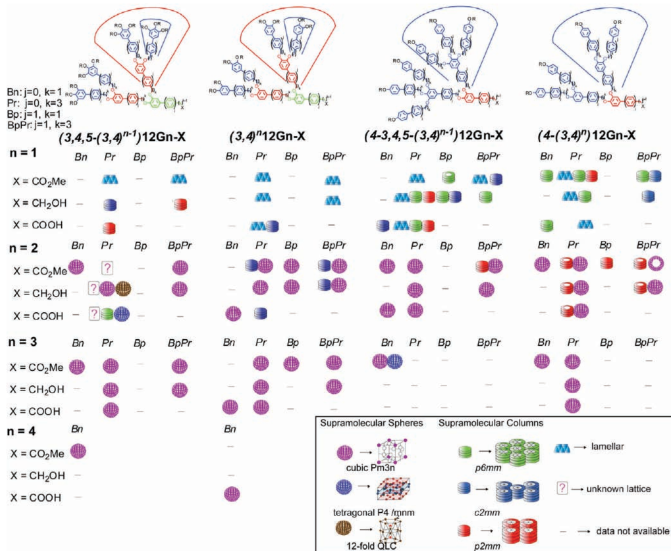
Figure 13. Primary structure vs 3D supramolecular structure relationship for all 3,4-disubstituted libraries of AB 2 supramolecular dendrimers. Bn = benzyl ether, Pr = phenylpropyl ether, Bp = biphenyl-4-methyl ether, BpPr = biphenylpropyl ether.
