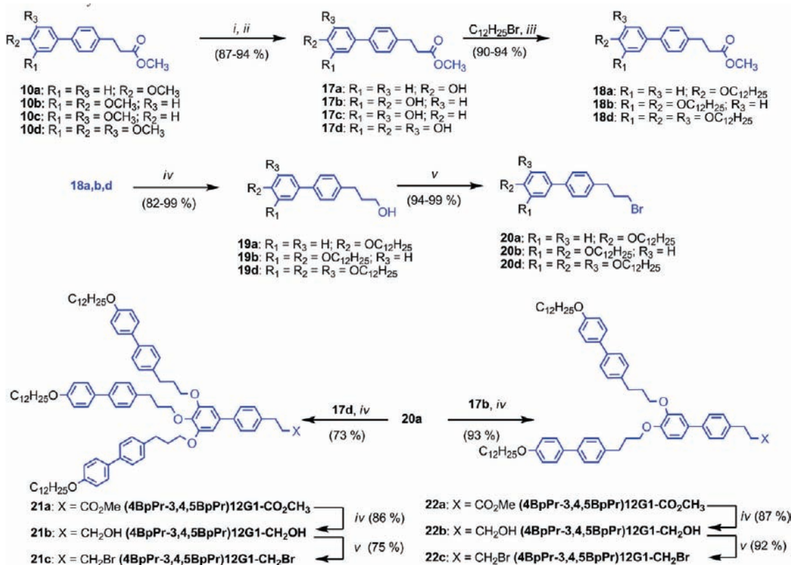
Scheme 4. Synthesis of First Generation Dendrons a
