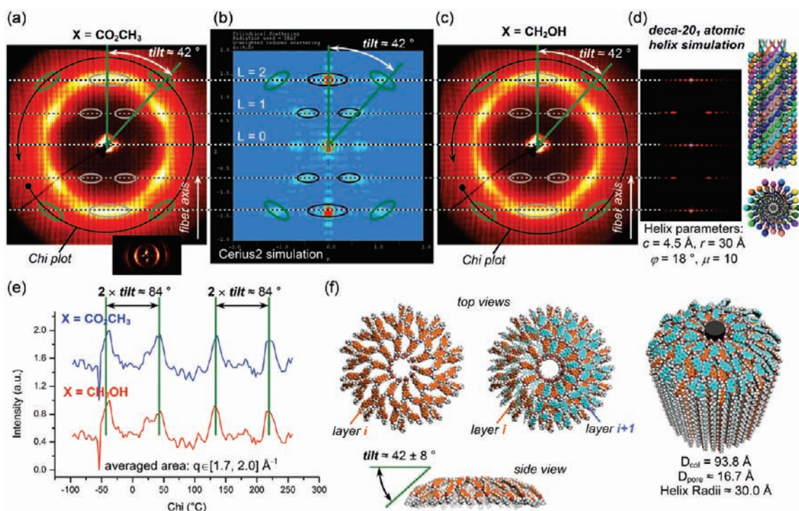
Figure 10. Supramolecular crown conformations assembled from (4BpPr-(3,4BpPr) 2 )-12G2-X (X = CO 2 CH 3 and CH 2 OH) and their self-organization into helical pyramidal columns. Wide-angle XRD oriented fiber patterns collected at 25 °C for X = CO 2 CH 3 (a), compared with the Cerius2 simulated diffraction pattern based on the corresponding molecular models of (4BpPr-(3,4BpPr) 2 )-12G2-CO 2 CH 3 (b), wide-angle XRD oriented fiber pattern collected at 25 °C for X = CH 2 OH (c), and theoretical diffraction pattern for a deca-20 1 helix (d). Azimuthal Chi angle plots along the region indicated on the fiber patterns (e). Molecular model for the X = CO 2 CH 3 (f). In (a, c): L indicates helical layer line; tilt indicates dendron tilt angle or tilt correlation features (marked in green); long-range helical features are marked by the gray colored circles.
