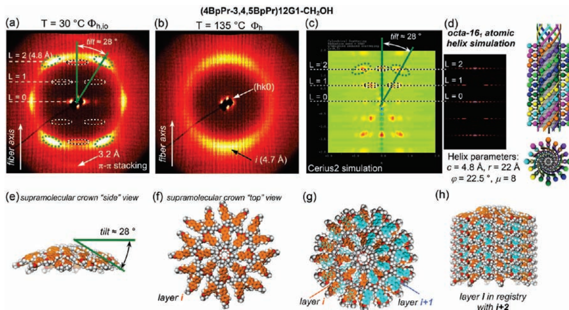
Figure 11. Wide-angle oriented fiber XRD patterns of the supramolecular columns assembled from the dendritic alcohol (4BpPr-3,4,5BpPr)12G1-CH 2 OH collected in the \Phi_{h,lo} phase (a) and \Phi_h phase (b). Cerius2 molecular model based simulation of the XRD pattern of the oriented fiber (c). Atomic helical packing, helix parameters, and the corresponding simulated XRD pattern (d) of the same supramolecular assembly. The molecular model of the supramolecular structure generated from (4BpPr-3,4,5BpPr)12G1-CH 2 OH used in the Cerius2 simulation (e, f, g, h).
