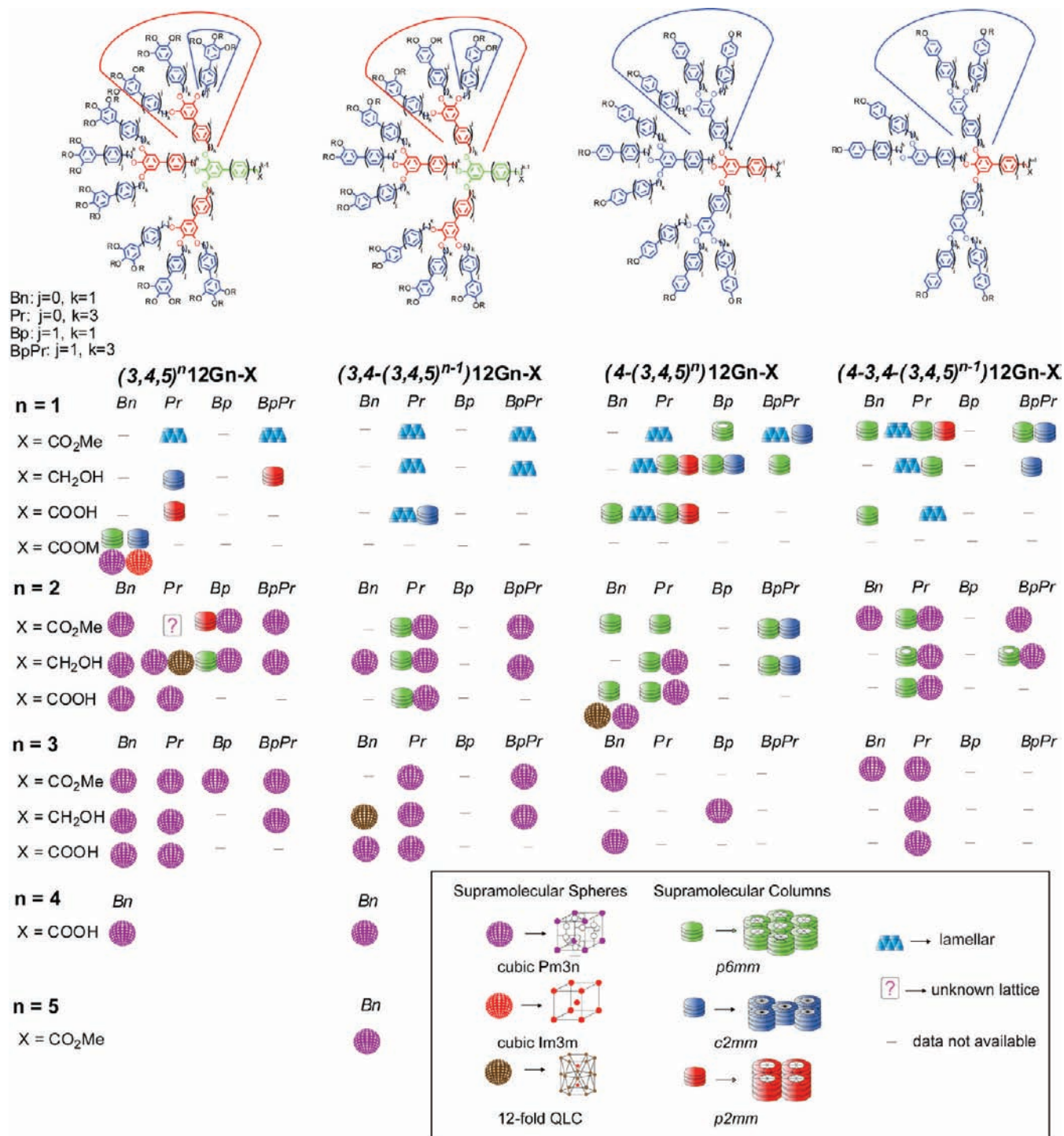
Figure 12. Primary structure vs 3D supramolecular structure for all libraries of AB 3 supramolecular dendrimers. Bn = benzyl ether, Pr = phenylpropyl ether, Bp = biphenyl-4-methyl ether, BpPr = biphenylpropyl ether.
