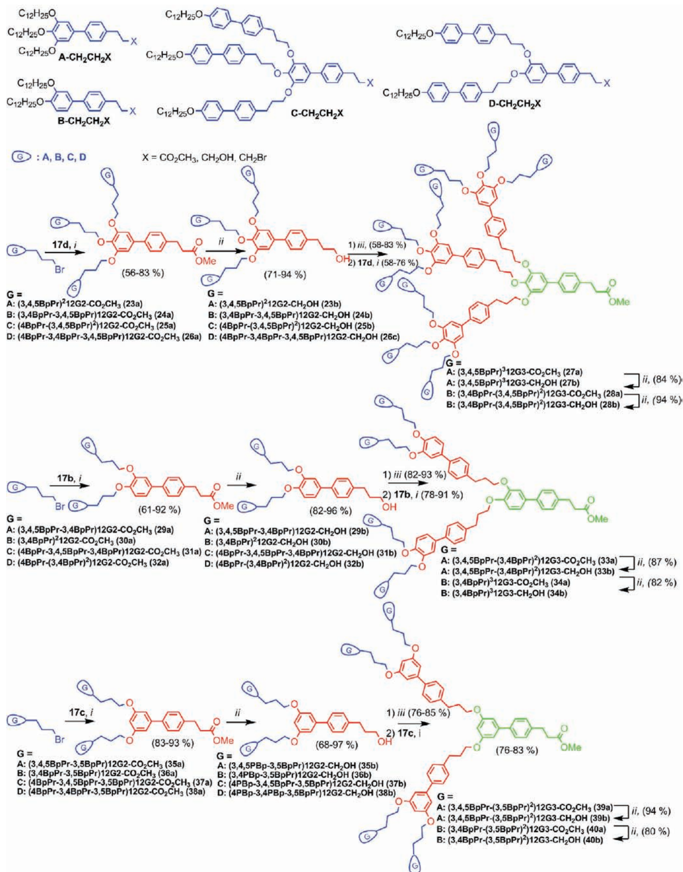
Scheme 5. Synthesis of Higher-Generation Dendrons a
