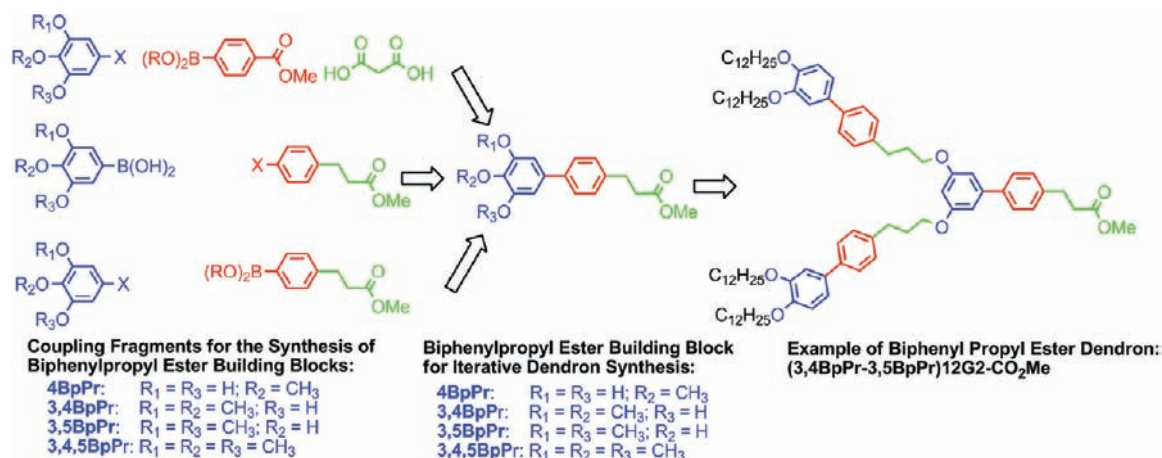
Figure 1. Three modular approaches to BpPr building blocks.
