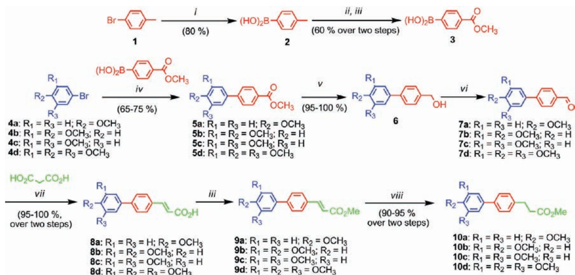
Scheme 1. Nine Step, Three Component Synthesis of BpPr Dendritic Building Blocks a
