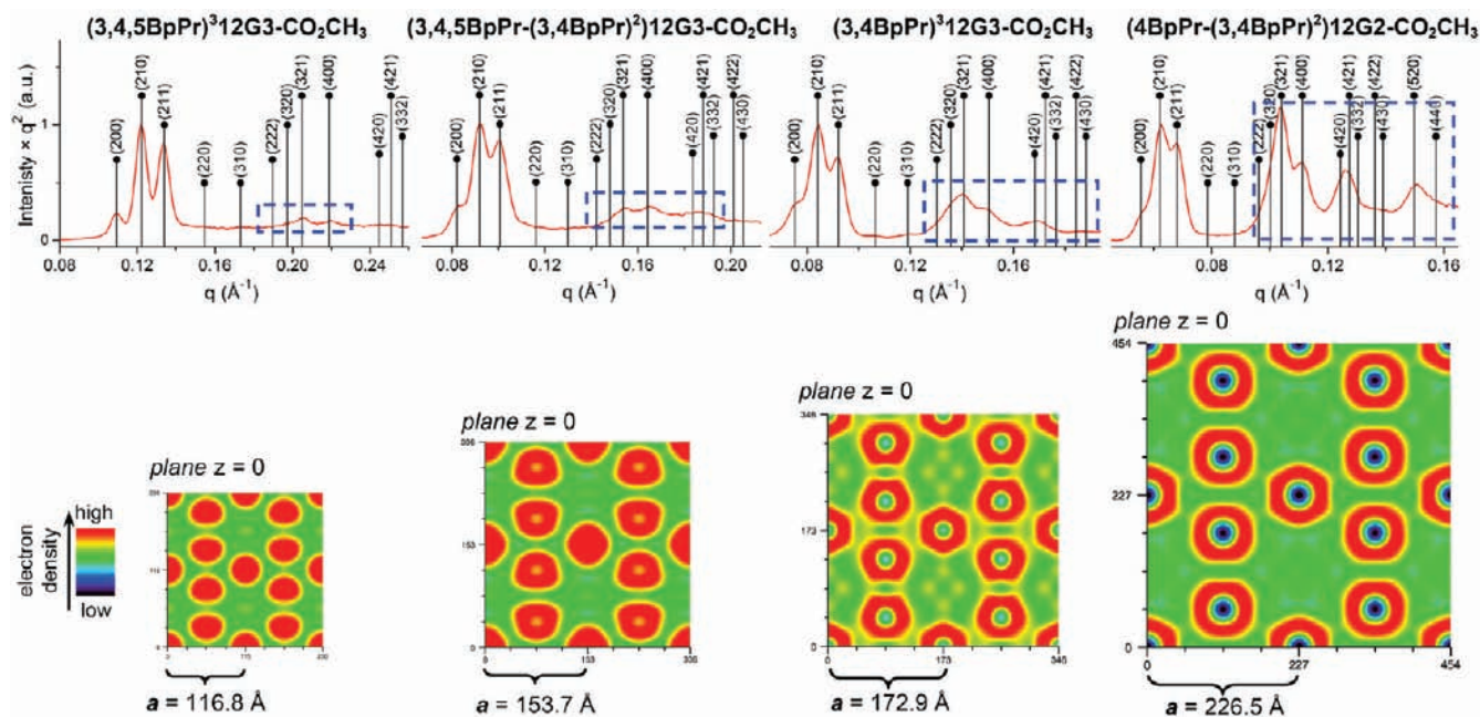
Figure 6. Small-angle powder XRD plots for selected BpPr dendrons that self-assemble into the Pm\bar{3}n cubic phase (top) and the corresponding reconstructed electron density maps, presented at relative scale (bottom). The dashed blue rectangles mark the increased intensity of the higher order diffraction peaks.
